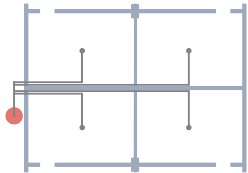
VSN 200 Multi-zone technology - saves space and extinguishing agent
