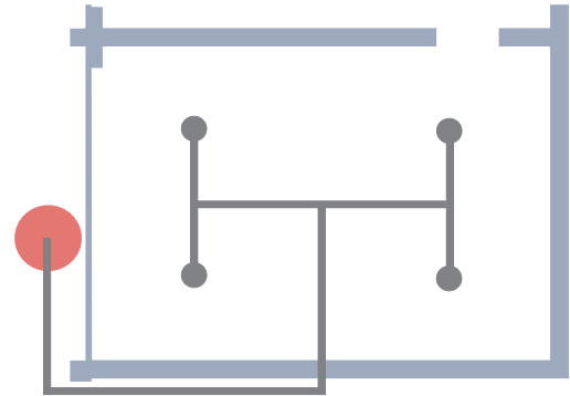
VSN 1230 50 bar technology - makes it possible to use long pipeworks
